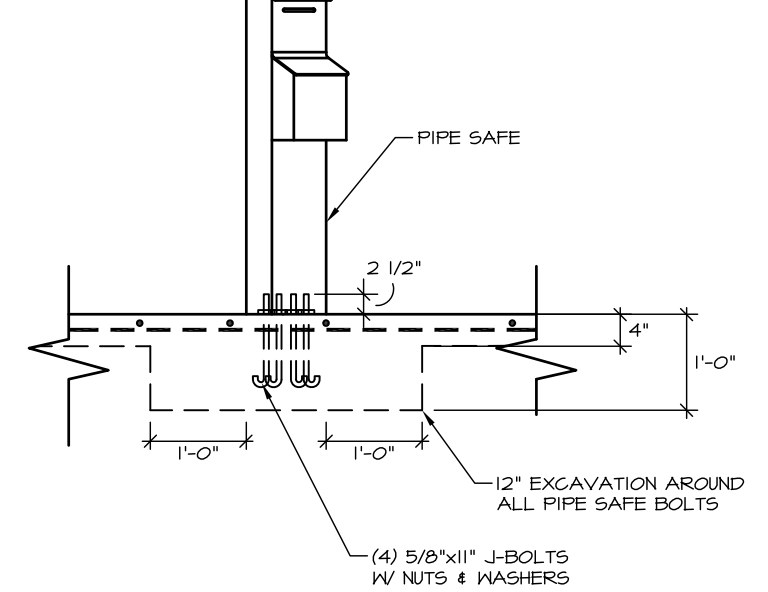
PIPE SAFE DETAILS
