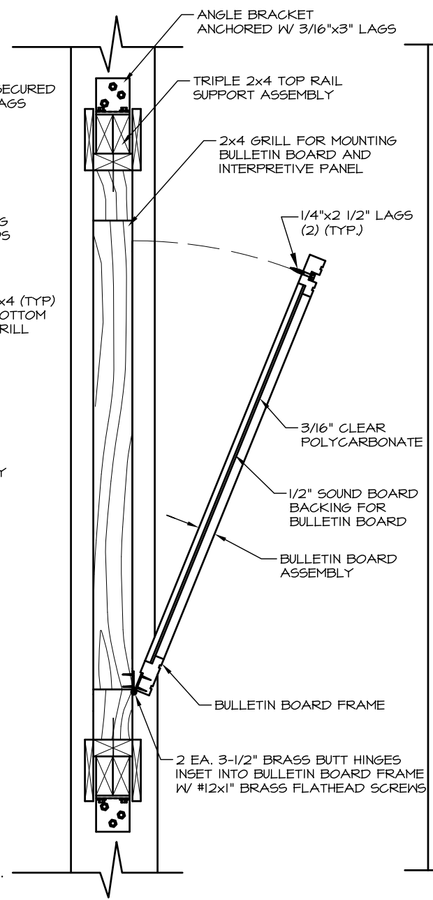
BULLETIN BOARD SECTION
