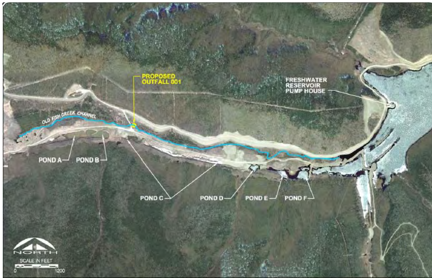
Figure 3: Enhanced Aerial Photo of the Outfall Location
