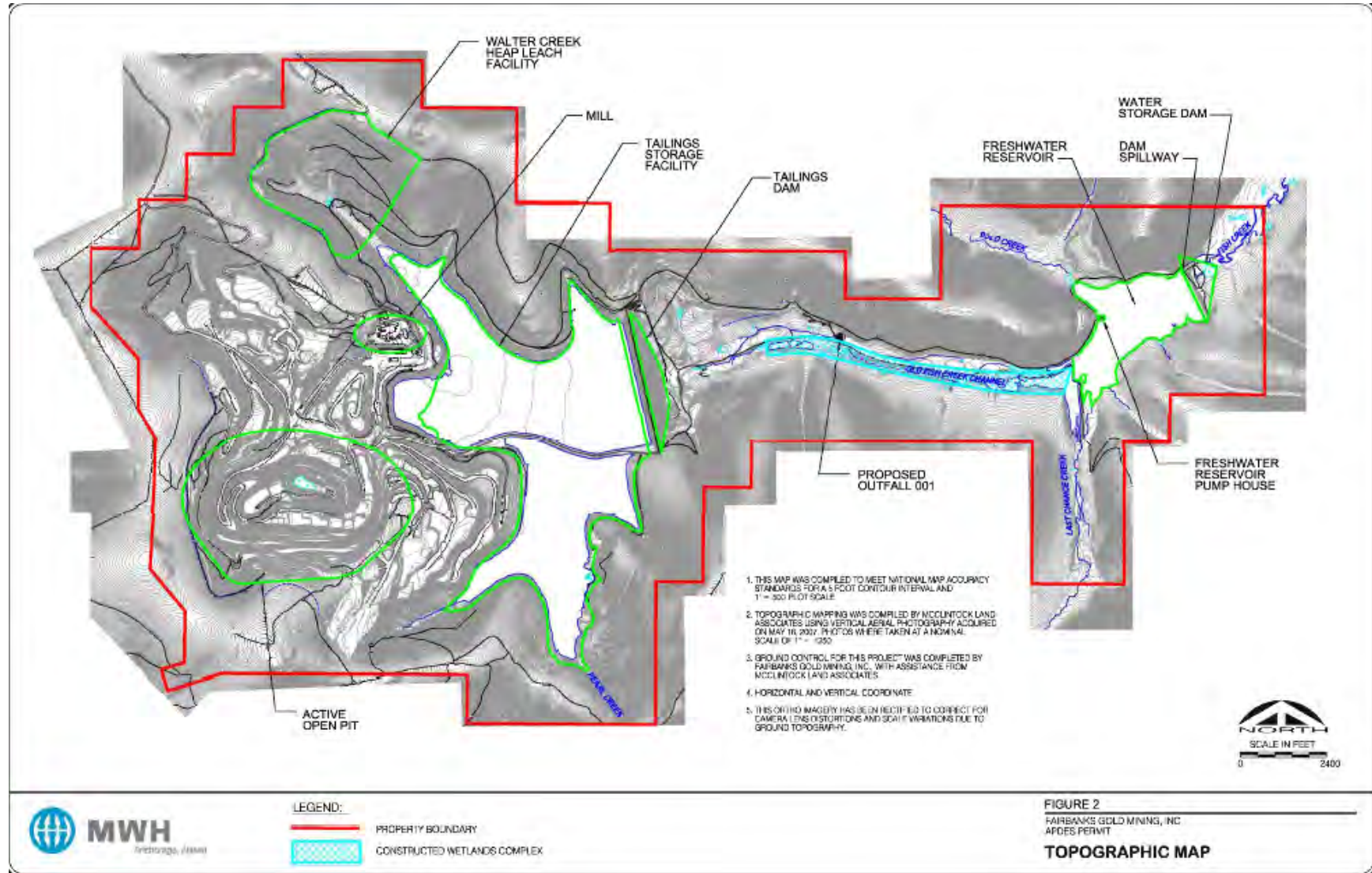
Figure 2: Facility Plan View Map
