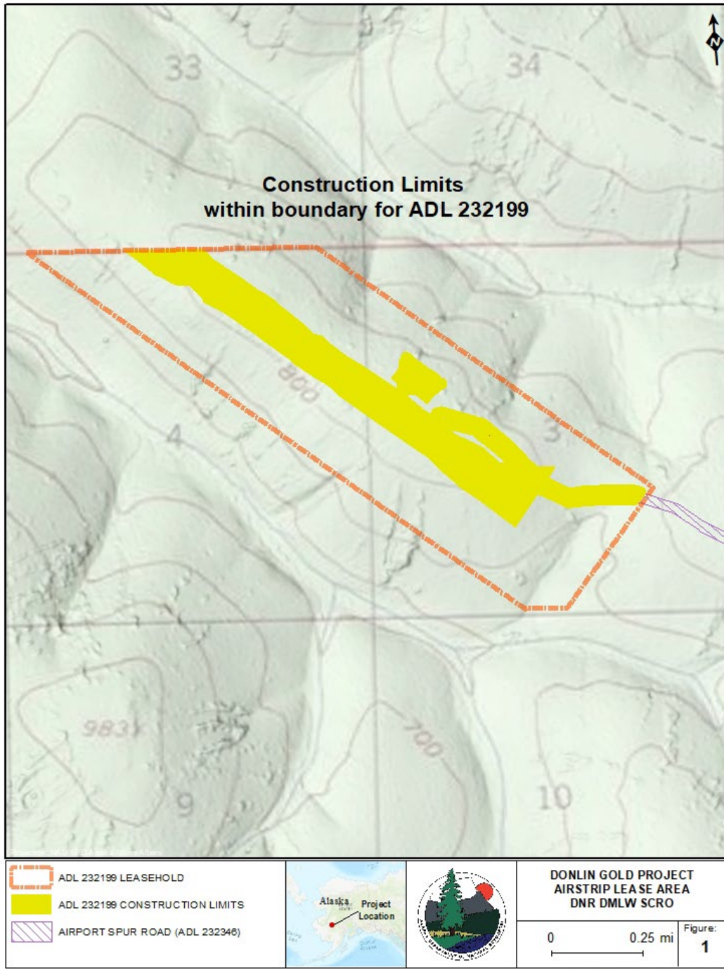
Figure 1: Construction limits for ADL 232199.
