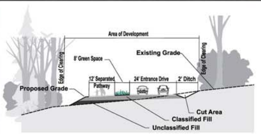
Entrance Road Section Typical
