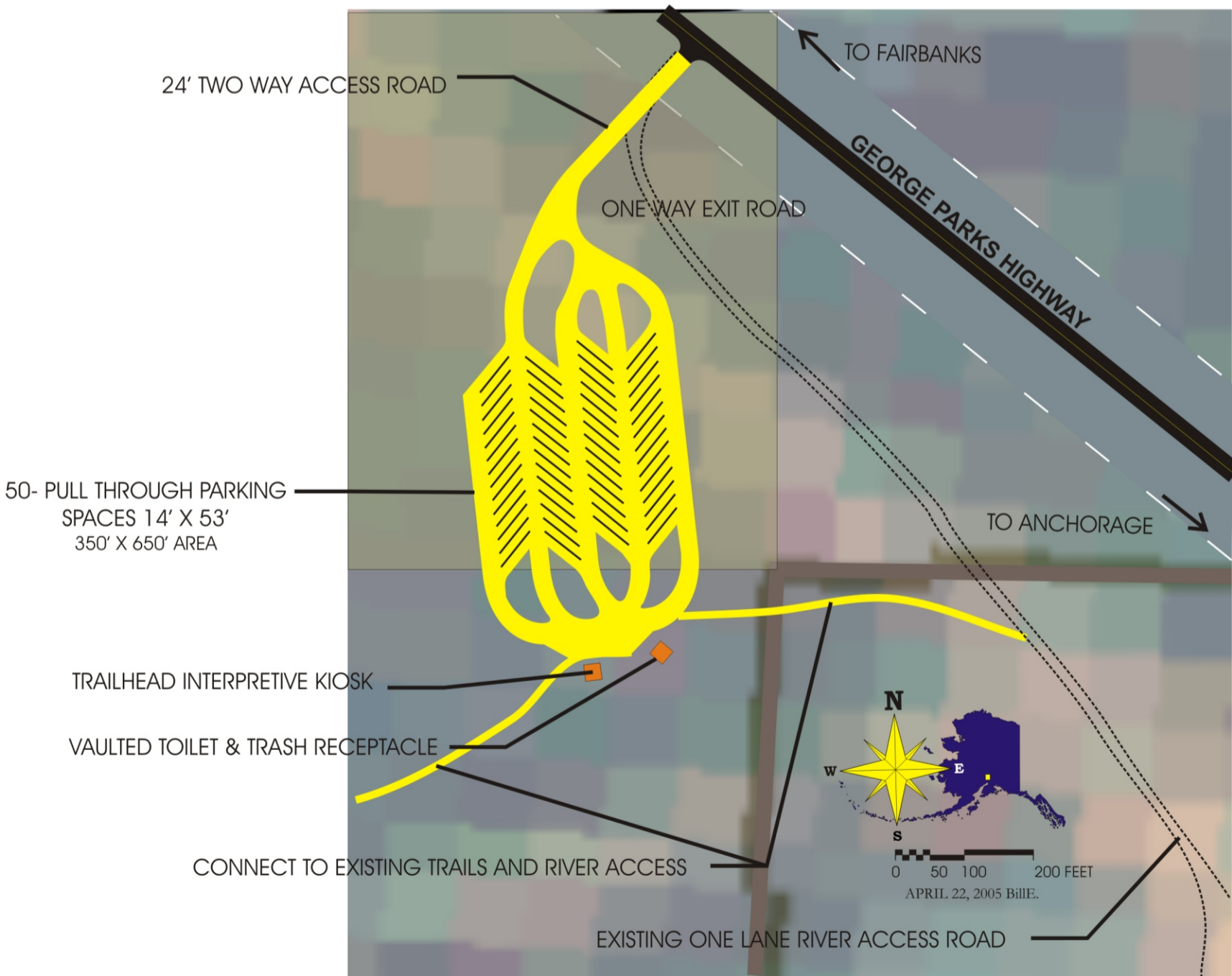
South Denali Rabideux Creek Parking Area SITE PLAN CONCEPT Map drawing is conceptual. Actual facility locations could change after thorough site investigations are conducted. Figure 2-3
