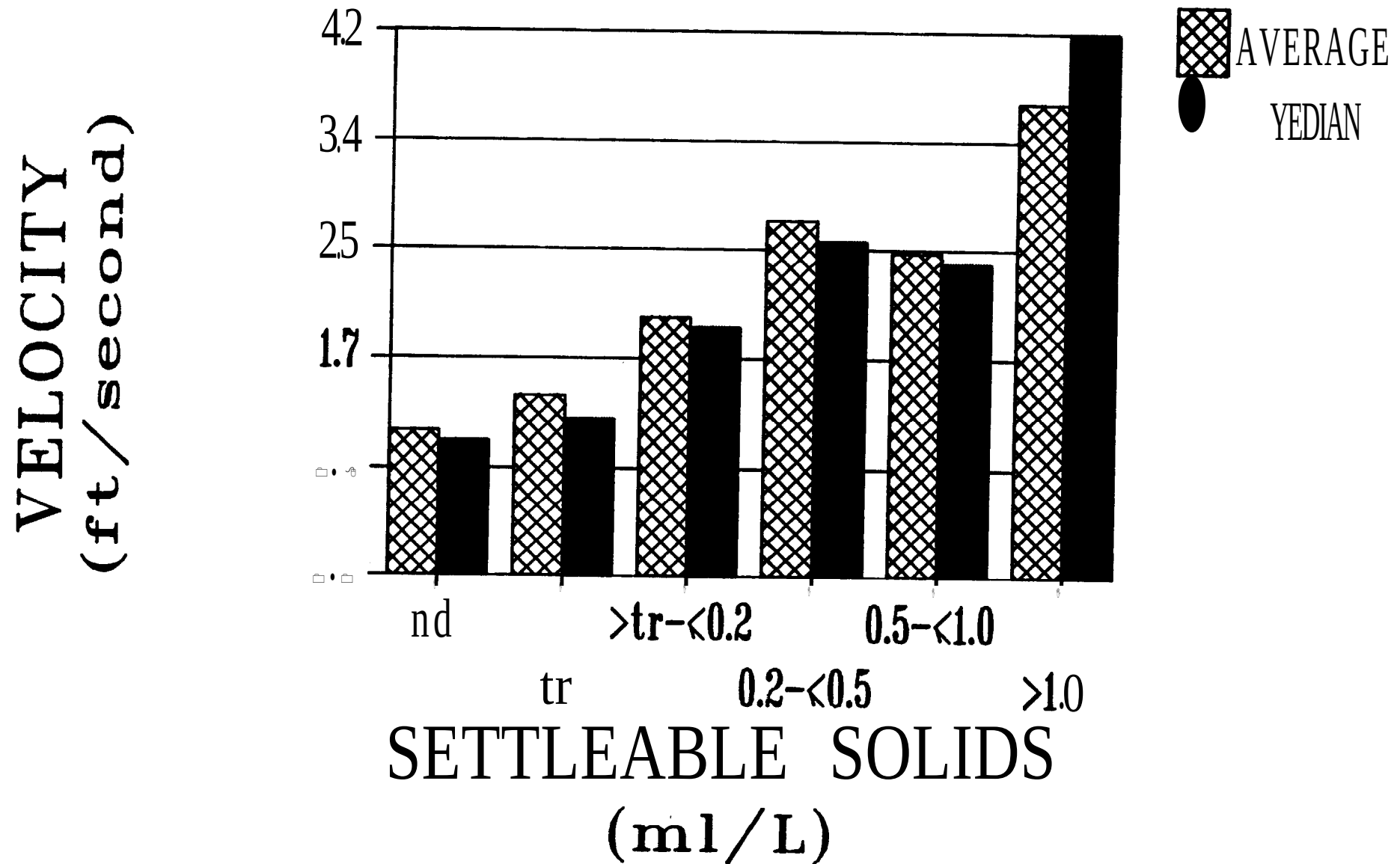
Figure 4. Velocity - settleable solids relationship
