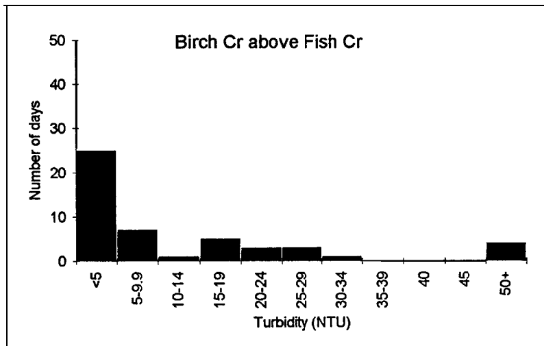
Figure 3. Frequency distributions of the turbidity data for seven of the automated sampling sites. Data are from samples collected from July 17 through September 5.
