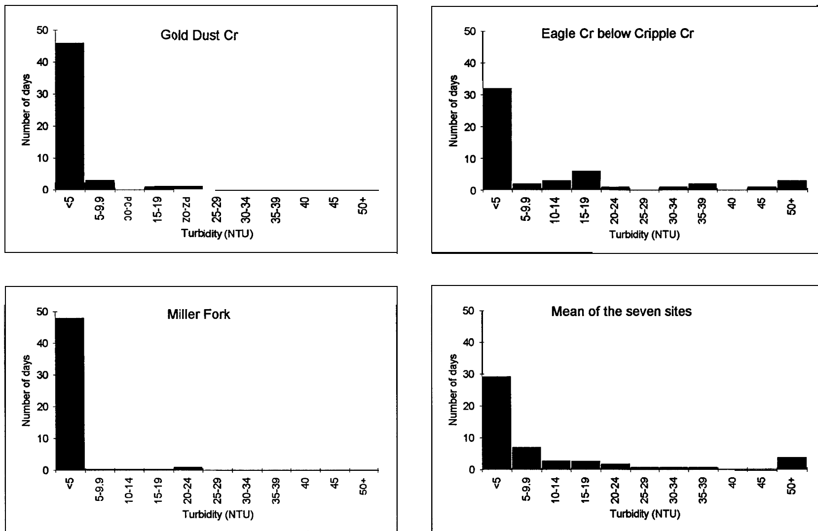
Figure 4. Frequency distributions of the turbidity data for seven of the automated sampling sites. Data are from samples collected from July 17 through September 5.
