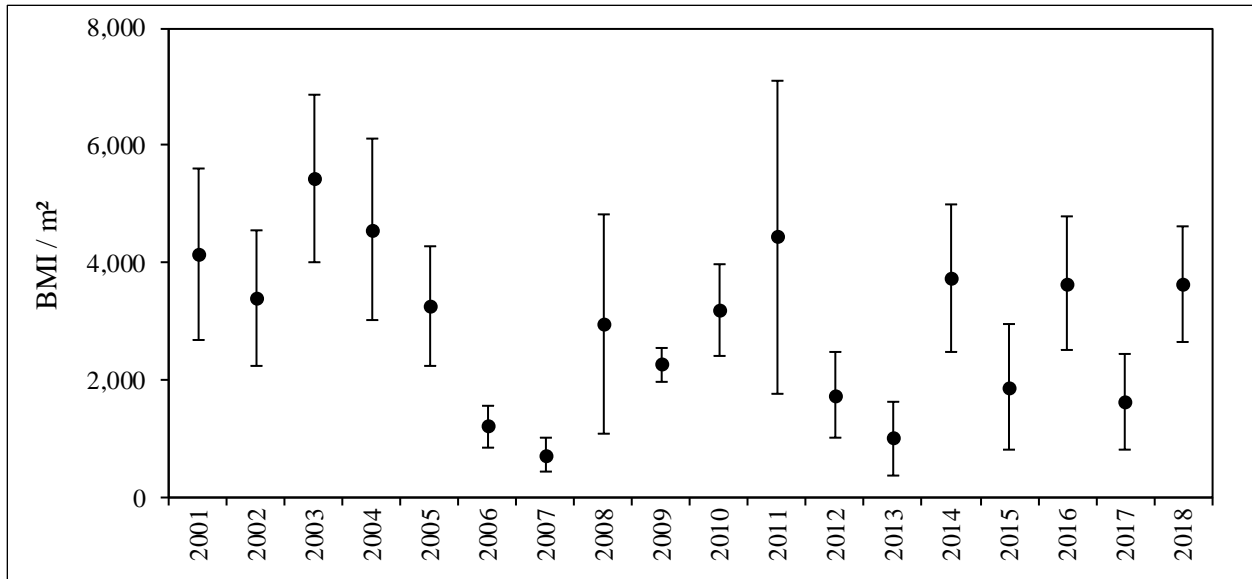
Figure 25.—Greens Creek Site 54 mean benthic macroinvertebrate densities \pm 1 SD.
