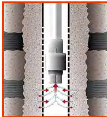
Figure 17.1.1: Cross Section of Waterra® Foot Valve
